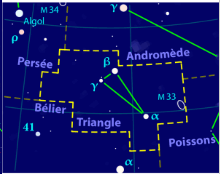
Triangle
