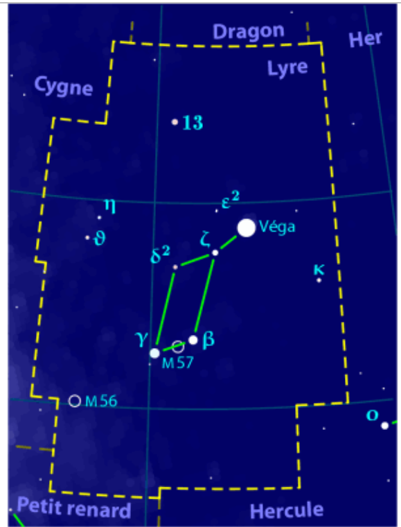
Lyre
