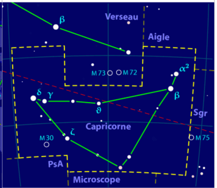
Capricorne
