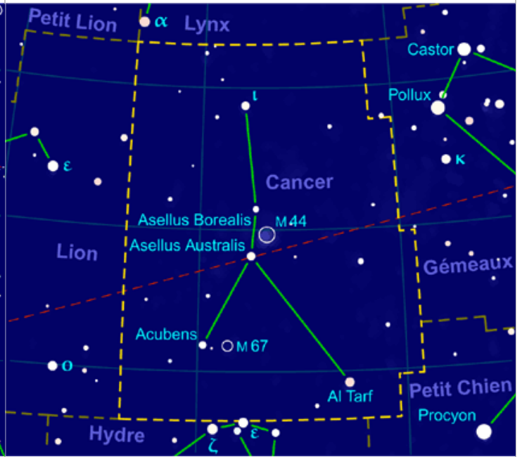
Cancer
