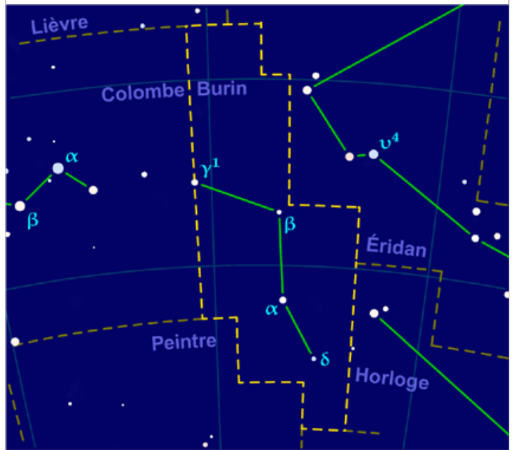
Burin
