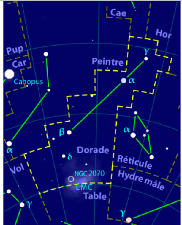
Dorade
