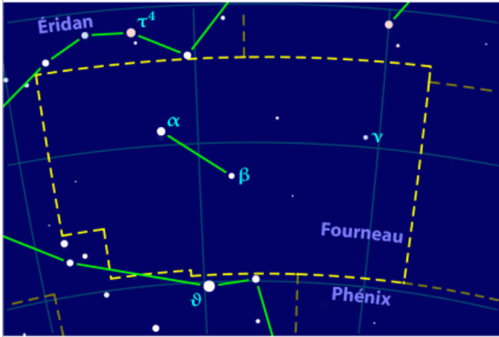
Fourneau
