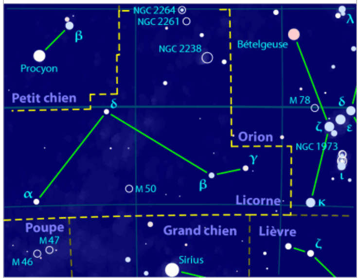
Licorne
