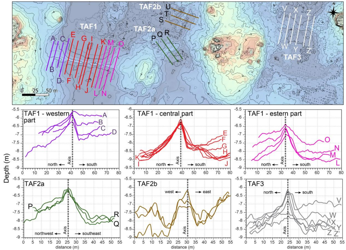
Figure 4. Cross-sections of the four main structures of Toul ar Fot (TAF1, TAF2 and TAF3). The position of the sections on the map is indicated by colour lines and letters (Author).
