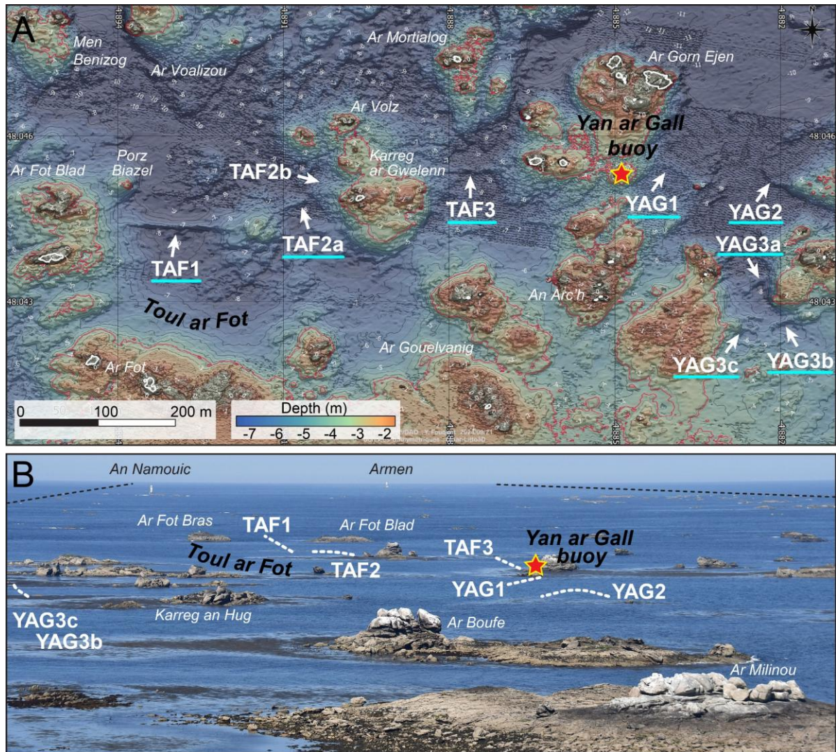
Figure 2. Toul ar Fot and Yan Ar Gall sectors. A: Bathymetric map and position of the Toul ar Fot (TAF) and Yann ar Gall (YAG) structures. See Figure 1 for the location of the map. Black elevation contours are spaced 0.5 m apart. Depths on the curves are given in metres above sea level (asl). The current coastline (thick white curve) and lowest astronomical tide level (red curve) are also displayed. The names underlined in turquoise blue indicate the walls that have been explored by dives. B: Panoramic view taken from the top of the Sein Island lighthouse, showing the reef line of Sein (see Figure 1) at low tide. The northern and southern boundaries of this granitic plateau are indicated by the gray dotted lines. The position of the structures explored during the dives is indicated by their name and by the white dotted lines. The names of the lighthouses and navigation towers are indicated in black (Authors).
