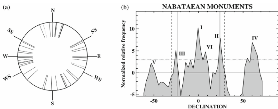
Fig. 4. Main outcomes of the archaeoastronomical analysis of Nabataean monuments. a, (left) orientation diagram of the structures (dot-lines for Roman period ones); b, (right) declination histogram of the set of monuments. Dashed and continuous vertical lines stand for major lunastices and solstices, respectively. Horizontal dot-line stands for the 3\sigma confidence level. Roman numbers identify peaks discussed within the text
