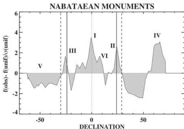
Fig. 5. Results yielded by a new analysis of the data in an attempt to test the significance of the peaks of accumulation. The observed declination histogram f(\text{obs}) is compared with the one that would be yielded by a uniform distribution of azimuths with the same number of data f(\text{unif}) and expressed in unit of the standard deviation of this second distribution. Peak IV is still significant within the distribution but peak V, which had already a low significance, loses all its weight
