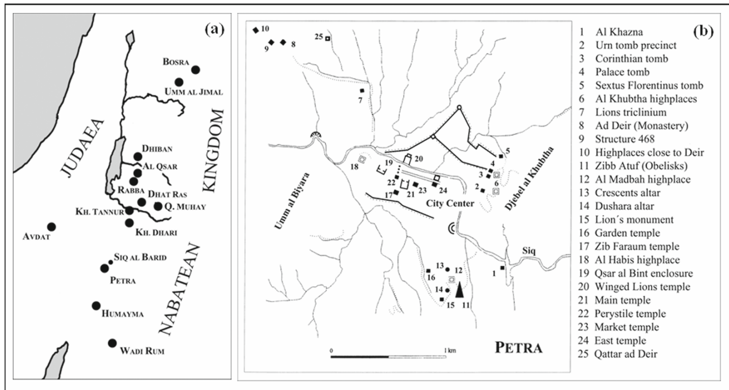
Fig. 1. Maps of the sites mentioned in the text and where the data have been collected: a) Sites of the Nabataean Kingdom discussed in the text; b) Sites of the city of Petra. Diagrams by the authors
