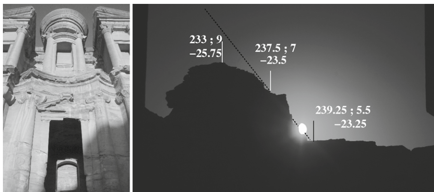
Fig. 6. Winter solstice sunset at Ad Deir: a, (left) the light and shadow effect in the innermost sacred area of the structure, the môtab ; b, (right) the accurate solstitial phenomenology associated with the site. Dotted line corresponds to the path followed during winter solstice sunset by the upper limb of the sun for the first century B.C. Photos: J. A. Belmonte and A.C. González-García, respectively
