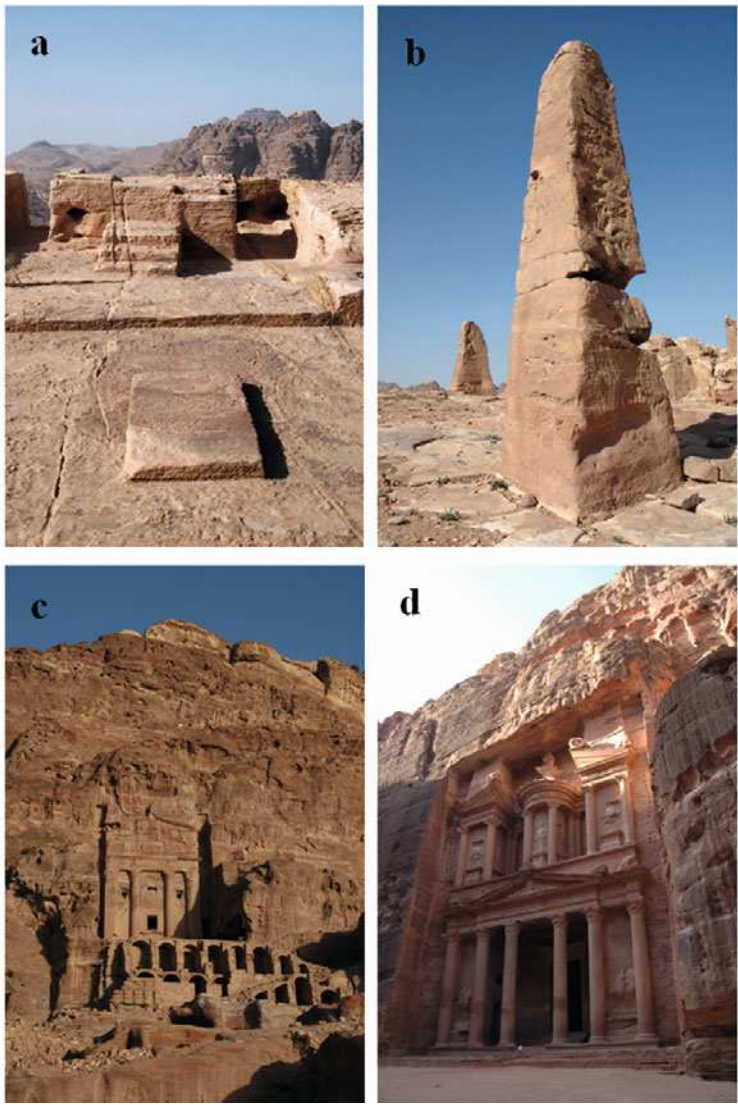
Fig. 2. Images of different kind of monuments of Petra measured, analyzed and discussed within the text: (a) Madbah highplace; (b) the Obelisks or Zibb Attuf at Djebel Madbah; (c) The Urn Tomb at the cliffs of Djebel Khubtha; and (d) the splendid façade of Al Khazna.
